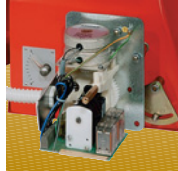
Example of servomotor for burners of PRESS T/N series
