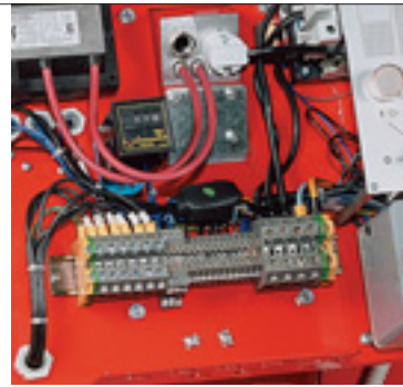
Example of the terminal board for electrical connections for P 140-200-300-450 T/N models
